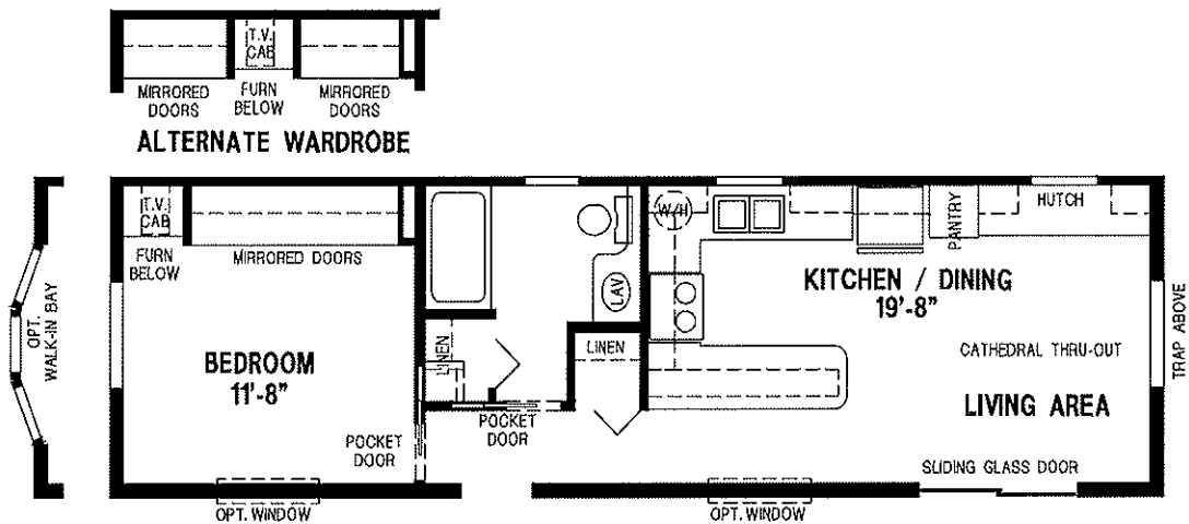
3027CTB/4012 1BEDROOM - CATHEDRAL THRU-OUT - SHED ROOF
